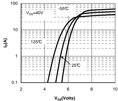
Figure 2: Transfer Characteristics
