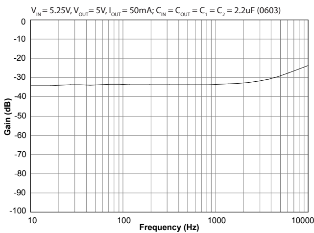
PSRR versus Frequency — 1x Mode
