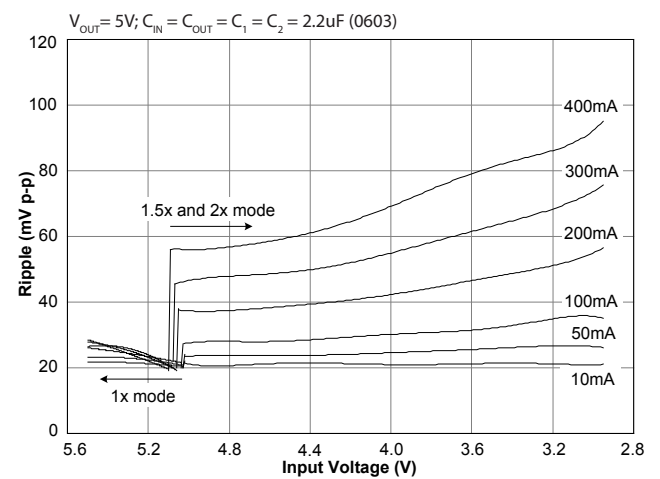
Output Ripple
