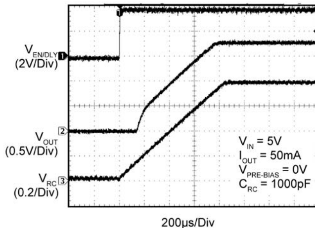
Figure 3. EN Turn-On Time – Normal Start-Up
