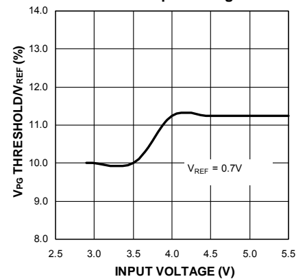
Power Good Threshold/ V_{REF} Ratio vs. Input Voltage
