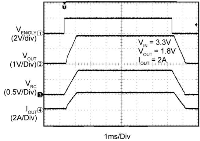
Enable Turn-On/Off
