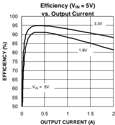
Figure 2. Efficiency Curve
