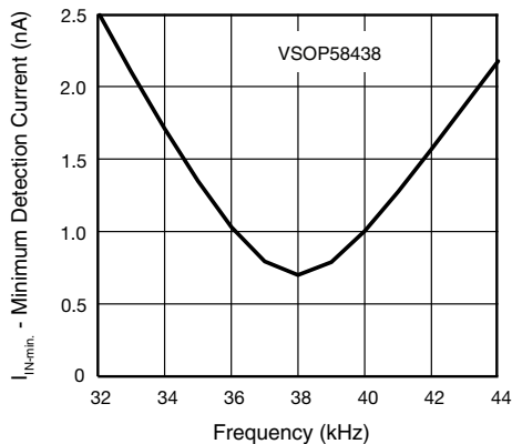
Fig. 4 - Bandpassfilter Characteristic
