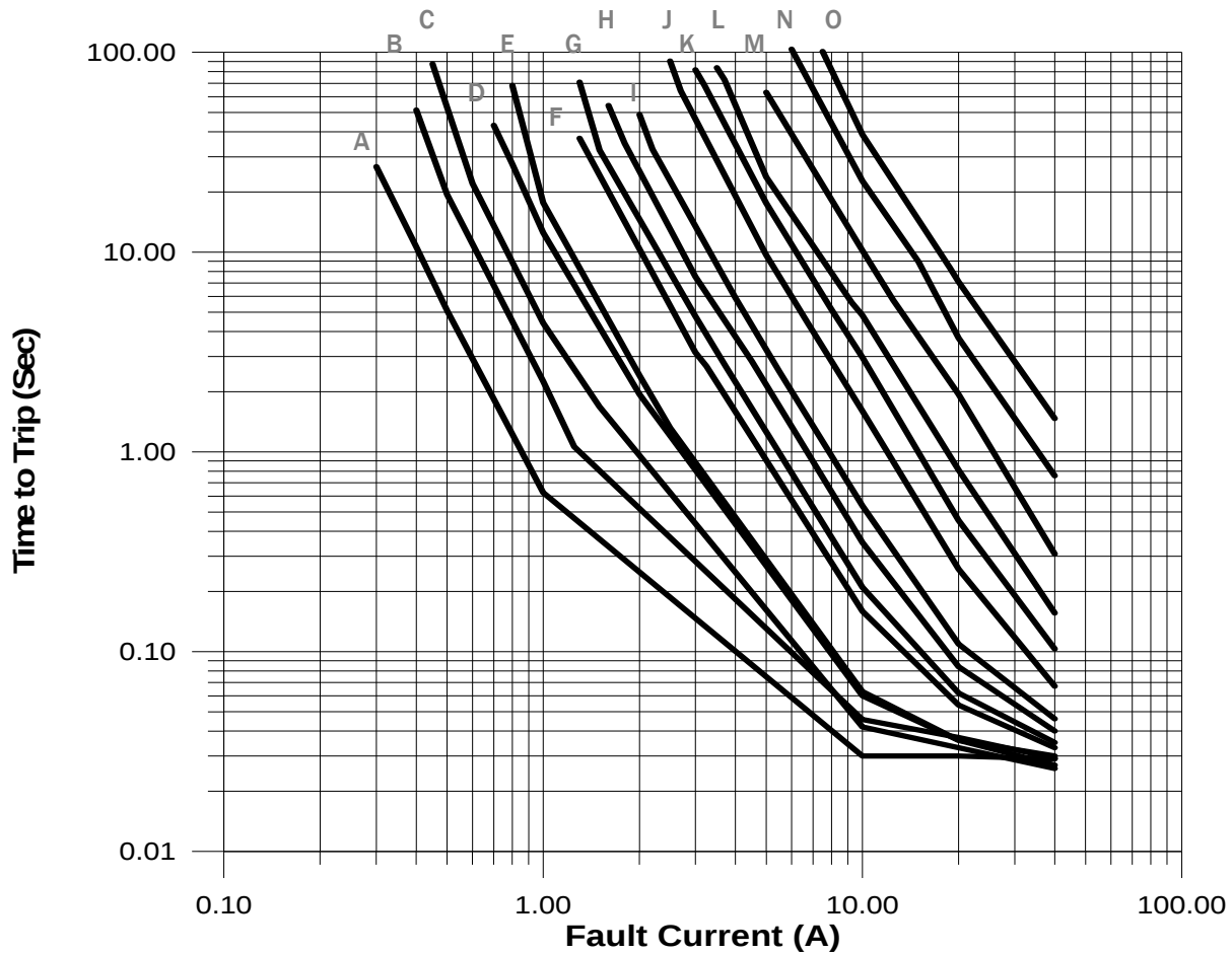
Average Time-Current Curve
