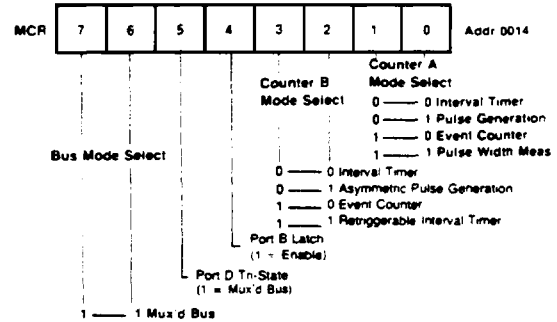
Mode Control Register
