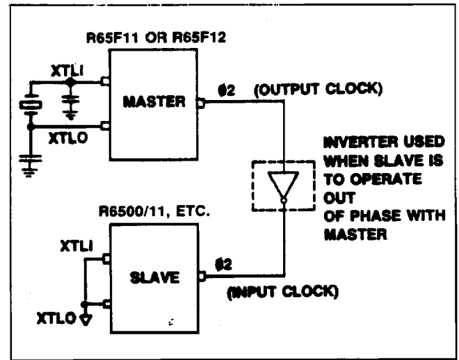
Figure 3-4. Master/Slave Connections
