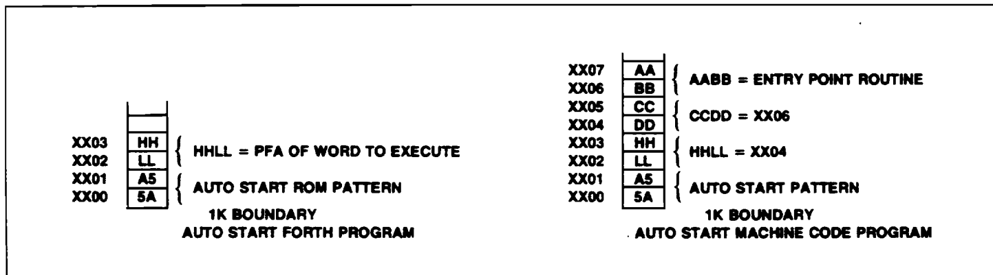
Figure 3-7. Auto Start ROM
