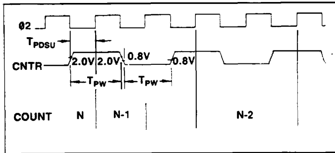
Figure 6-2. Event Counter Mode
