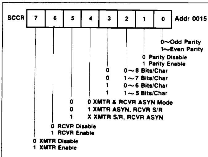
Figure 5-1. Serial Communication Control Register
