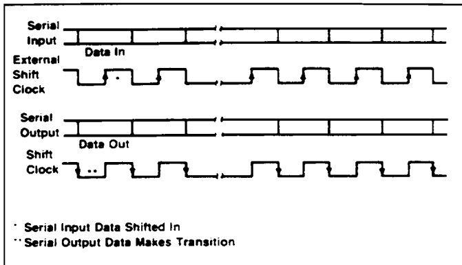
Figure 5-4. S/R Mode Timing
