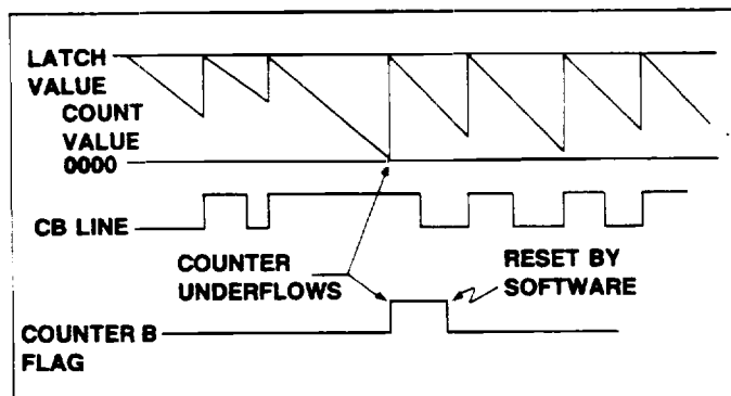
Figure 6-4. Counter B. Retriggerable Interval Timer Mode
