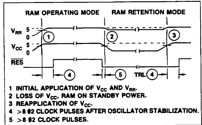
Figure 3-2. Data Retention Timing
