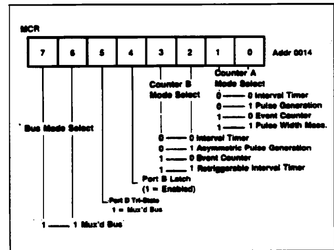
Figure 3-5. Mode Control Register
