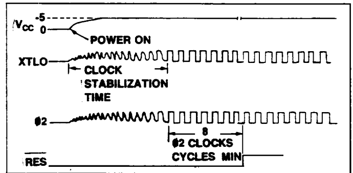
Figure 7-1. Power Turn-On Timing Detail
