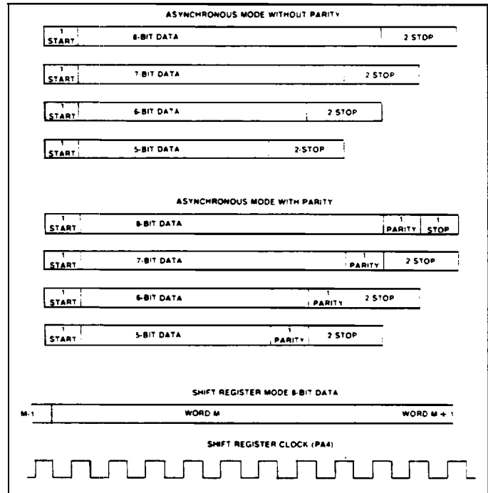
Figure 5-2. Bit Allocations
