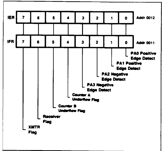
Figure 3-6. Interrupt Enable and Flag Registers
