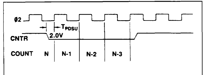
Figure 6-3. Pulse Width Measurement
