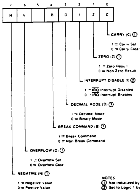
Processor Status Register
