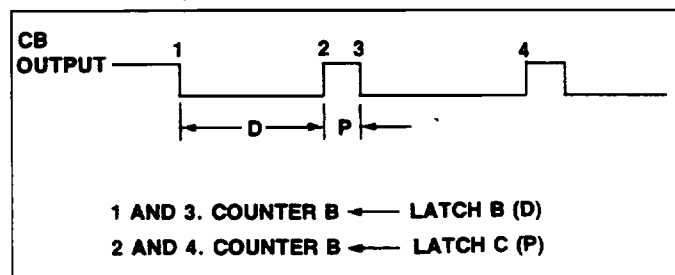
Figure 6-5. Counter B Pulse Generation
