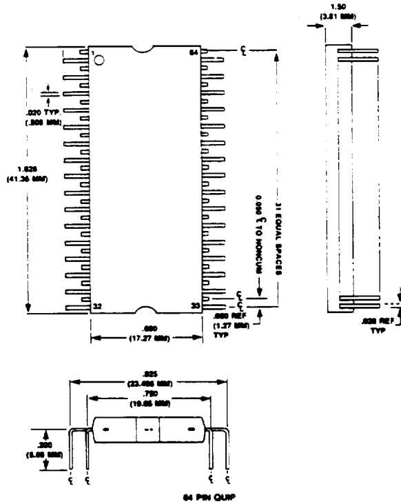
Figure 2-2. Pin Out Configuration
