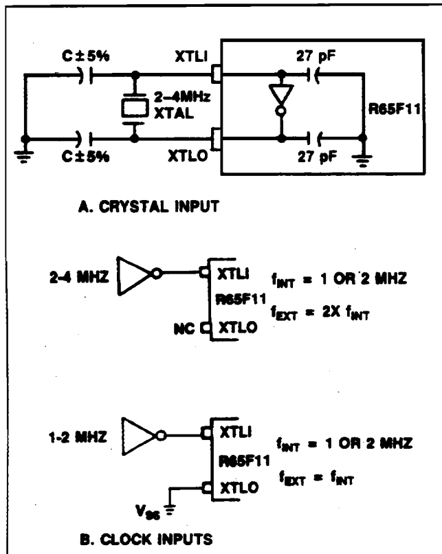
Figure 3-3. Clock Oscillator Input Options
