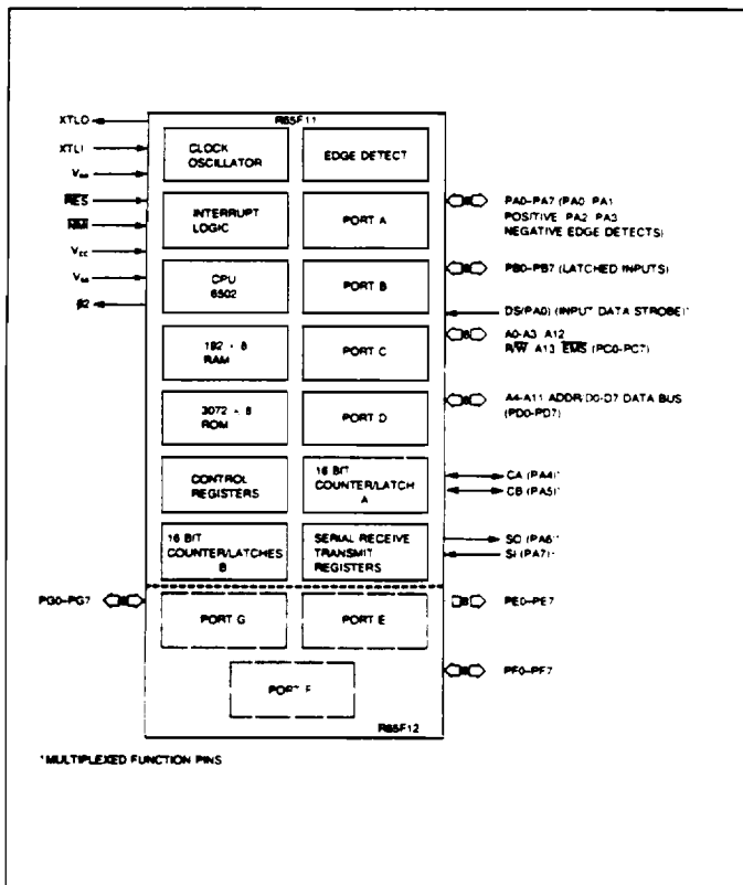
Figure 2-1. R65F11 and R65F12 Interface Diagram
