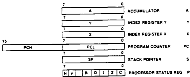
CPU Registers
