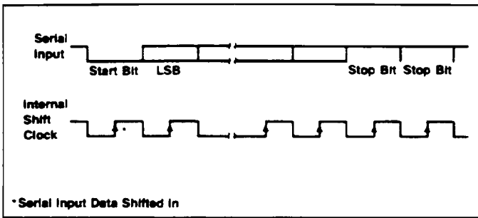
Figure 5-3. ASYN Receive Data Timing
