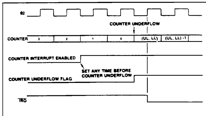
Figure 6-1. Interval Timer Timing Diagram
