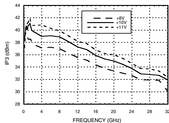
Output IP3 vs. Supply Voltage @ Pout = 16 dBm / Tone
