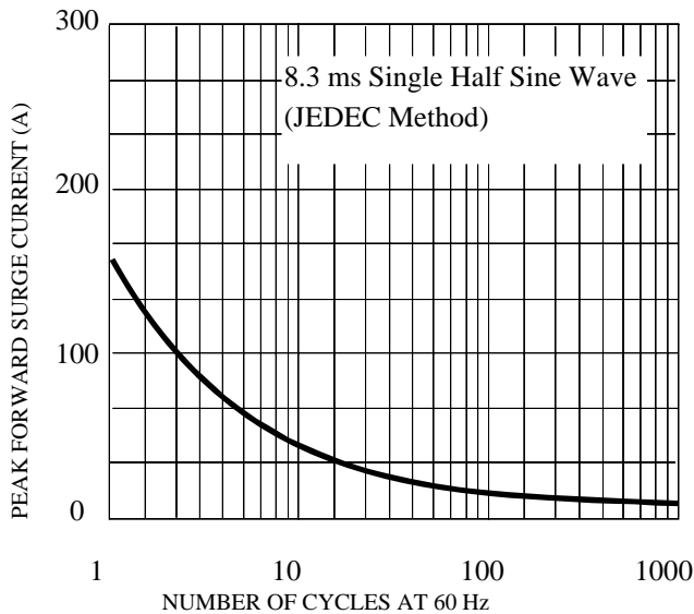
FIG. 5 -MAXIMUM NON-REPETITIVE FORWARD SURGE CURRENT
