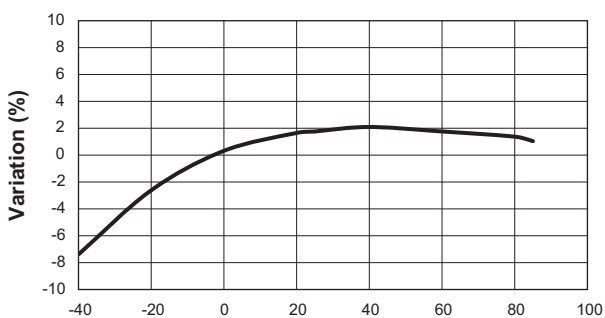
Switching Frequency Variation vs. Temperature
