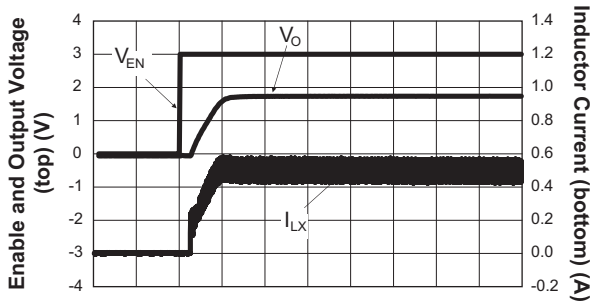
Soft Start
