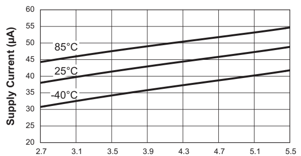
No Load Quiescent Current vs. Input Voltage
