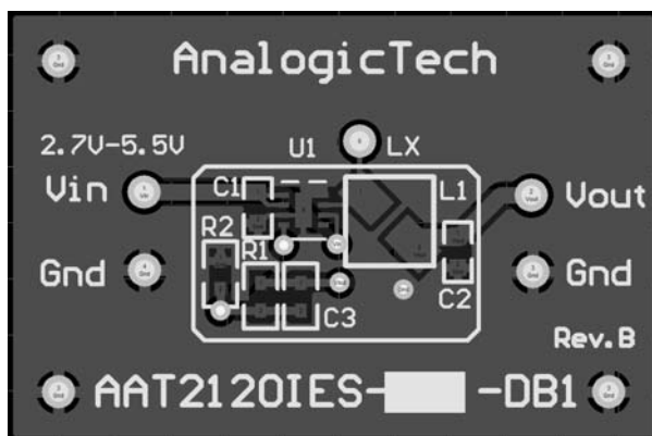
Figure 2: AAT2120 Evaluation Board Top Side Layout.
