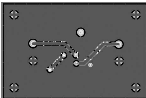
Figure 4: AAT2120 Evaluation Board Bottom Side Layout.
