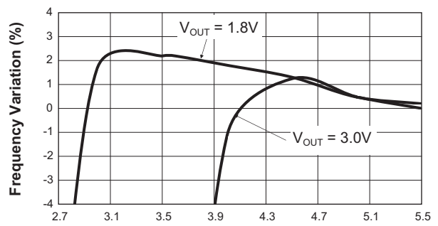
Frequency Variation vs. Input Voltage
