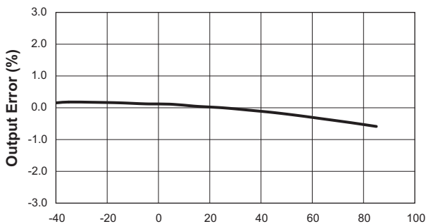
Output Voltage Error vs. Temperature
