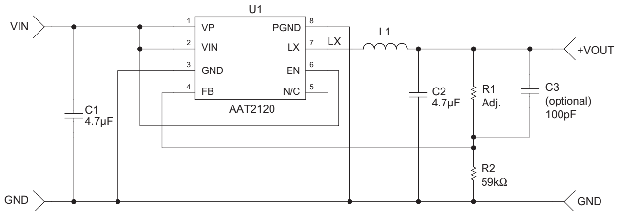
Figure 1: AAT2120 Schematic.
