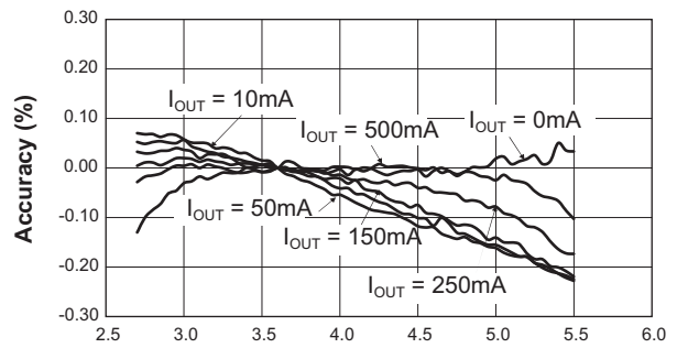
Line Regulation
