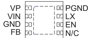
STDFN22-8 (Top View)
