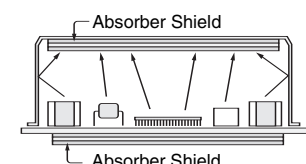
Absorbers shown in use below and above Printed Circuit Board.
