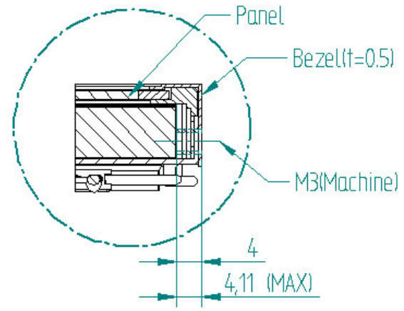
SEC. B-B
