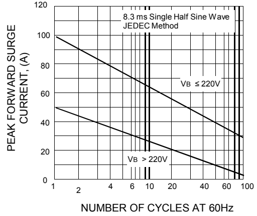
FIG.4 - PULSE RATING CURVE
