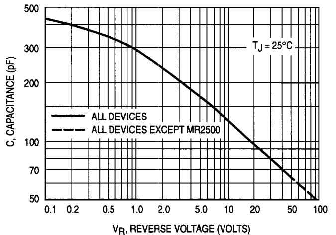
Figure 7. Capacitance
