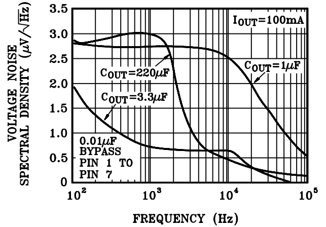
OUTPUT NOISE
