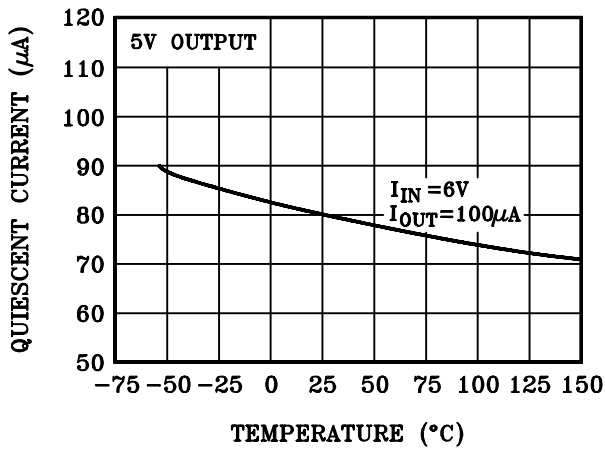
QUIESCENT CURRENT
