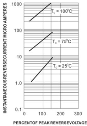
Fig.3-TYPICAL REVERSE CHARACTERISTIC
