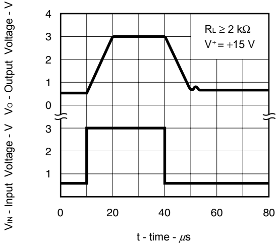
PULSE RESPONSE
