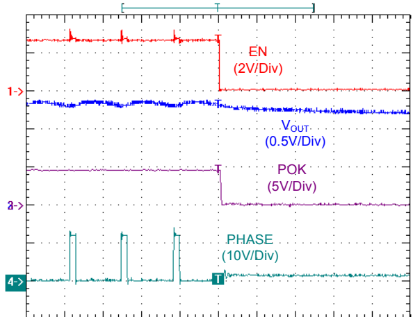
Time: 2.5us/Div V IN = 12V, V CC = 5V, I OUT = 2A
