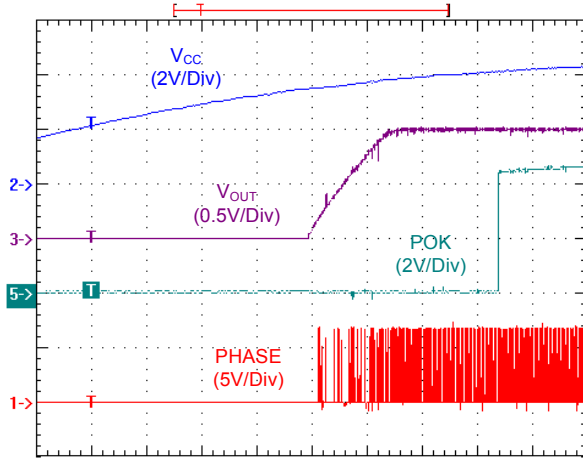
Time: 1ms/Div V IN = 7.0V, V CC = 5V
