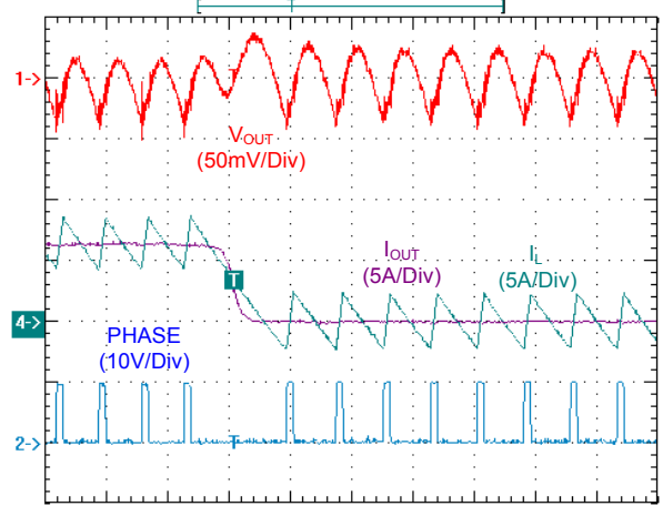
Time: 5us/Div V_{IN} = 10V, V_{OUT} = 1.5V, I_{OUT} = 8 \text{ to } 0A transient, FCCM
