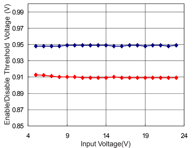
Enable/Disable Threshold Voltage vs. V IN
