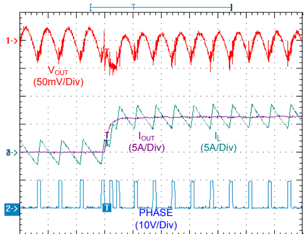
Time: 5us V IN = 10V, V OUT = 1.5V, I OUT = 0 to 8A transient, FCCM
