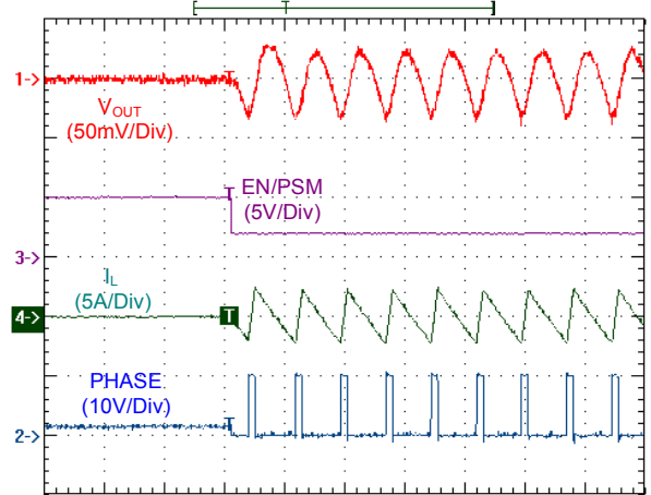
Time: 5us V_{IN} = 10V, V_{OUT} = 1.5V
