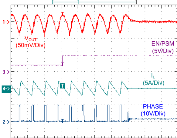
Time: 5us V_{IN} = 10V, V_{OUT} = 1.5V
