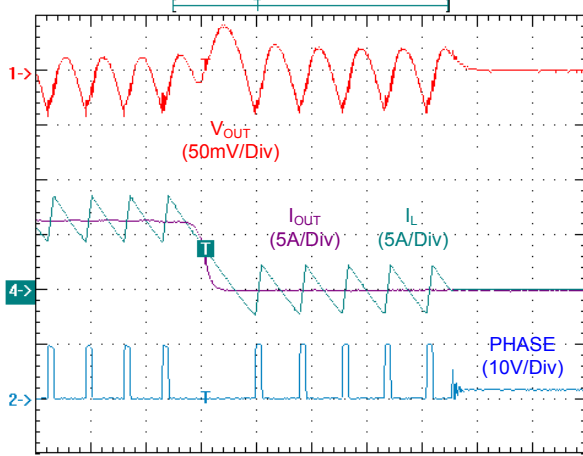
Time: 5us/Div V_{IN} = 10V, V_{OUT} = 1.5V, I_{OUT} = 8 \text{ to } 0A transient, PSM
