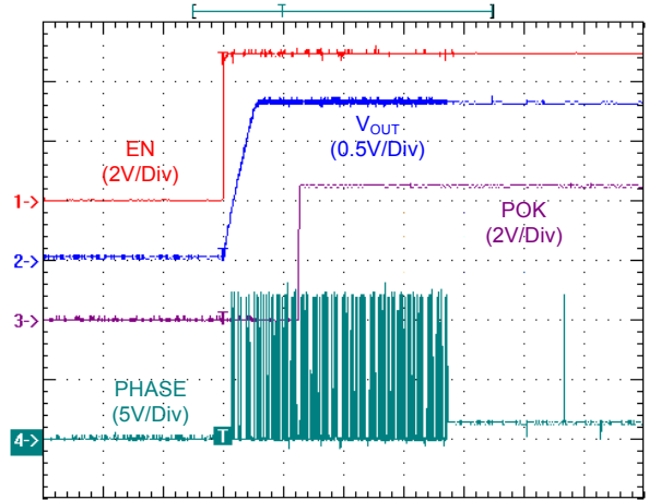
Time: 2.5ms/Div V IN = 12V, V CC = 5V
