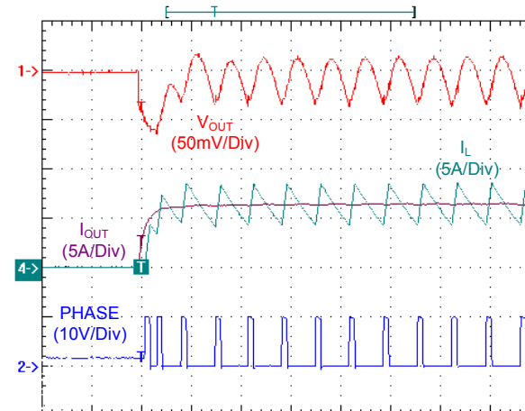
Time: 5us V IN = 10V, V OUT = 1.5V, I OUT = 0 to 8A transient, PSM
