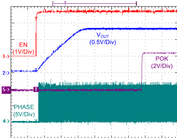
Time: 500us/Div V IN = 12V, V CC = 5V
