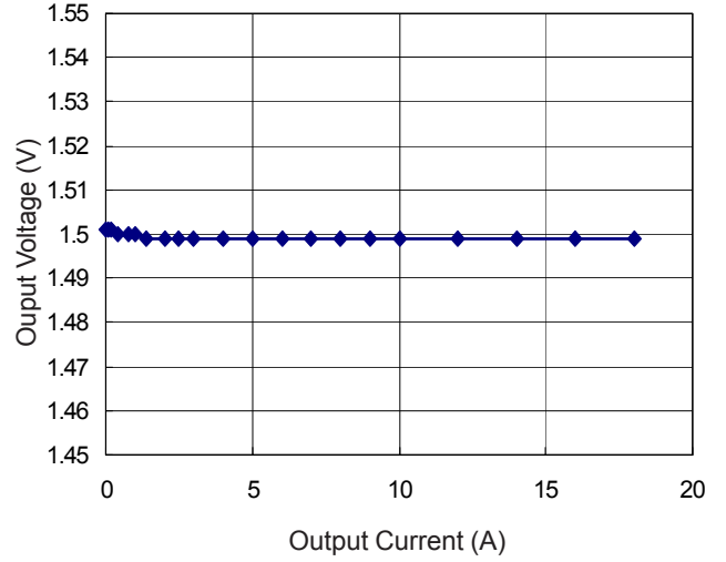
Load Regulation
