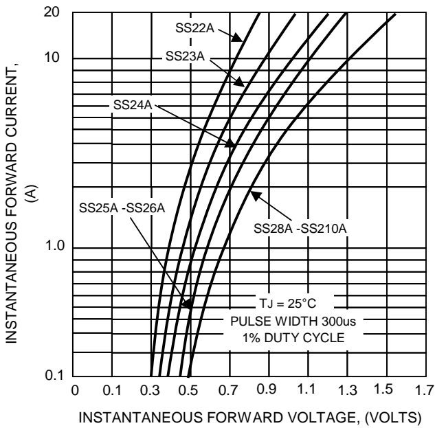
FIG.4-TYPICAL FORWARD CHARACTERISTICS
