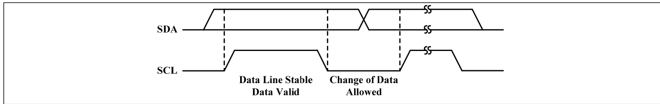
Figure 4 Interface timing
