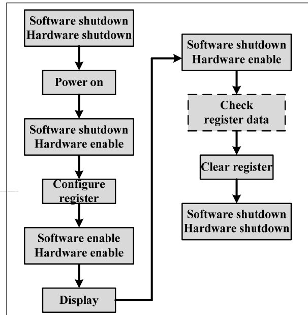
Figure 15 Shutdown Control
