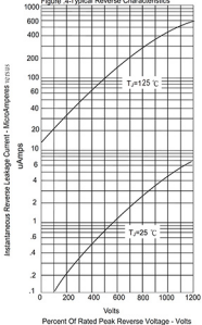
Figure 4-Typical Reverse Characteristics
