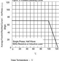
Figure 2- Forward Derating Curve
