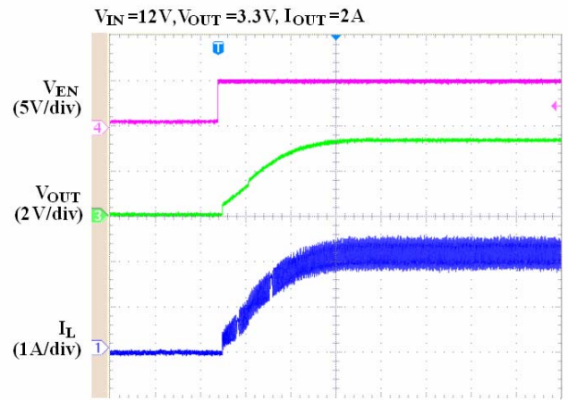
Times (4ms/div)
