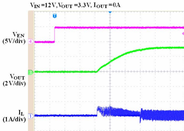
Times (100us/div)
