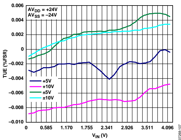
Figure 7. Total Unadjusted Error (TUE) vs. V_{IN}
