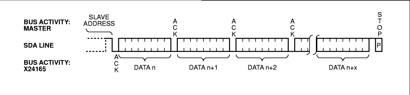
Figure 9. Sequential Read
