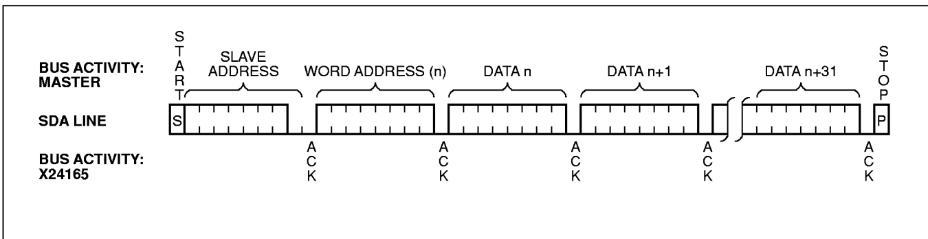
Figure 6. Page Write
