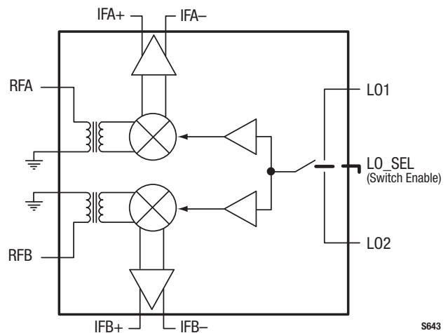
Figure 1. SKY73089-11 Block Diagram
