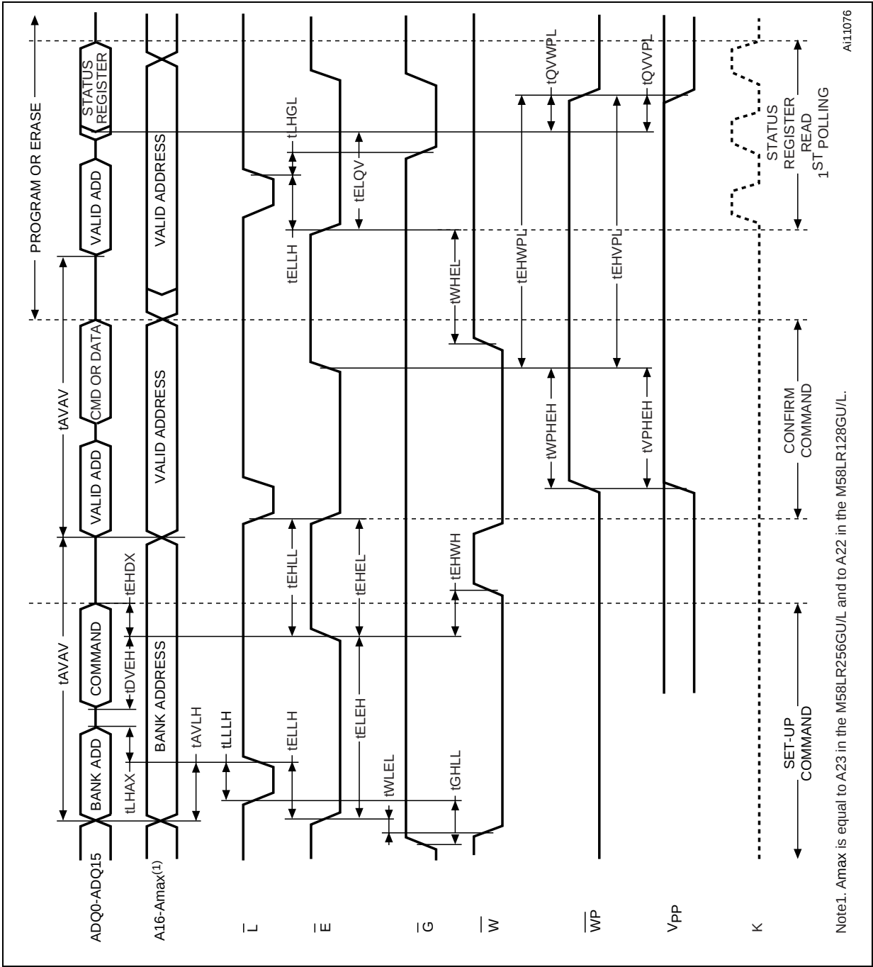
Figure 16. Write AC waveforms, Chip Enable controlled
