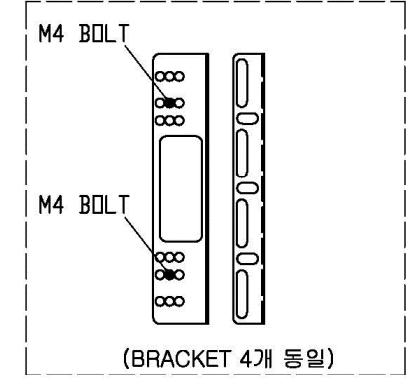
[19" BRACKET 체결방법]
