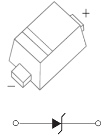
SOD-523
