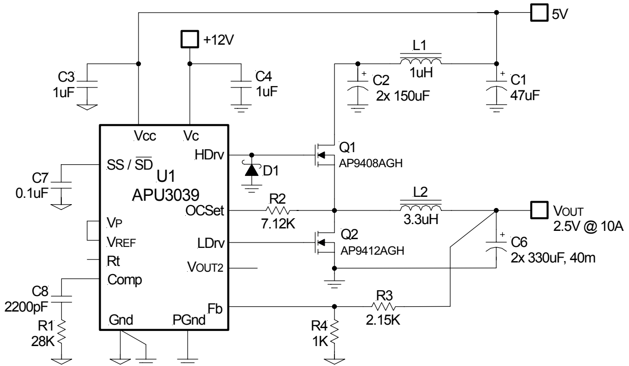
Figure 15 - Typical application of the APU3039 with two input supplies.
