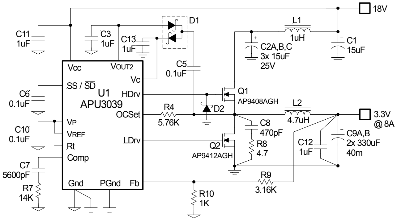
Figure 17 - Demo-board application of the APU3039.
