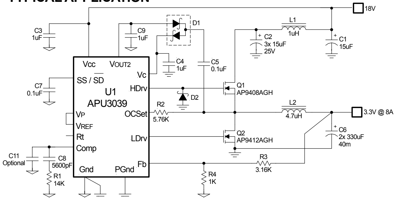
Figure 1 - Typical application of APU3039.
