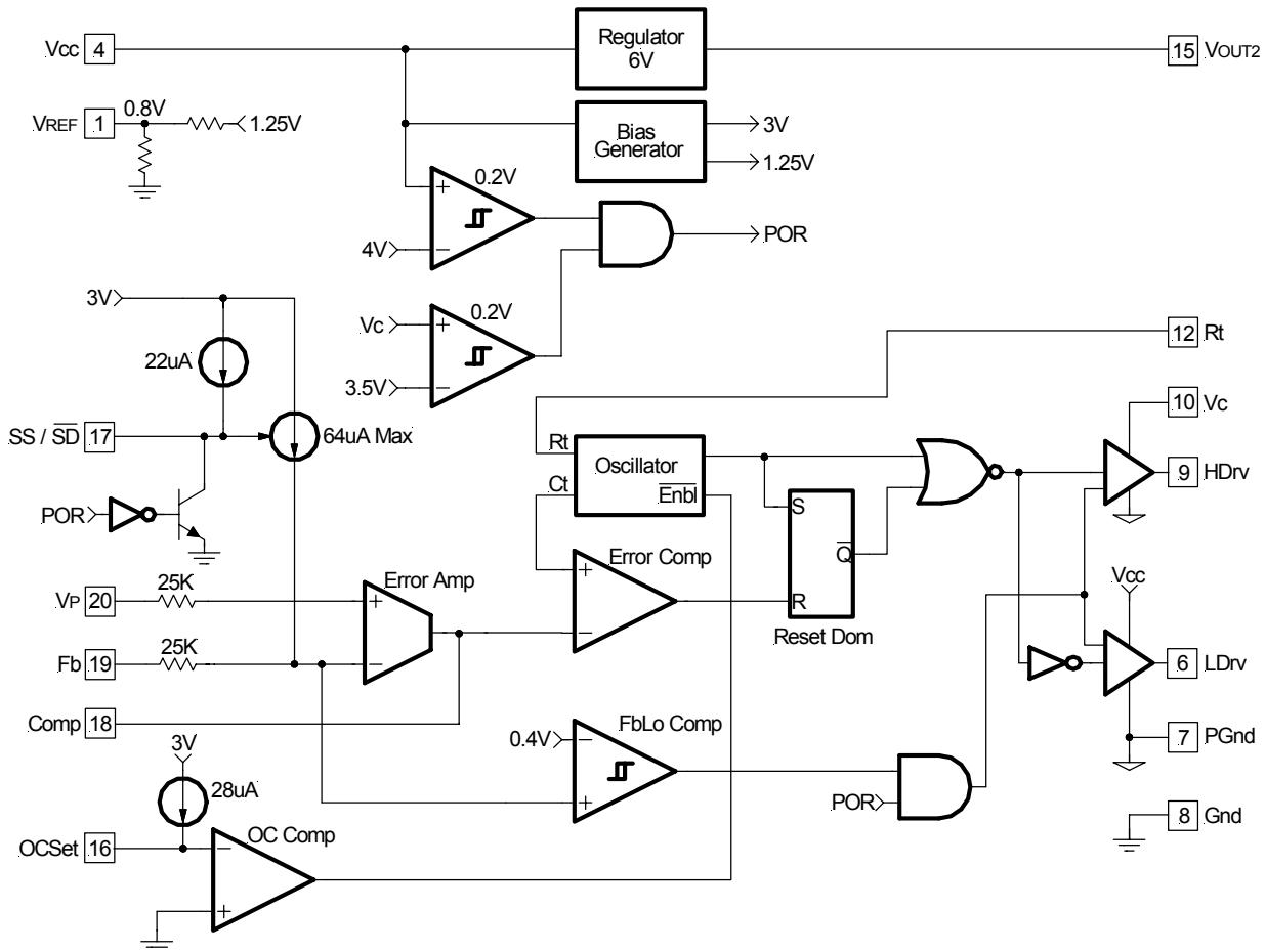
Figure 2 - Simplified block diagram of the APU3039.
