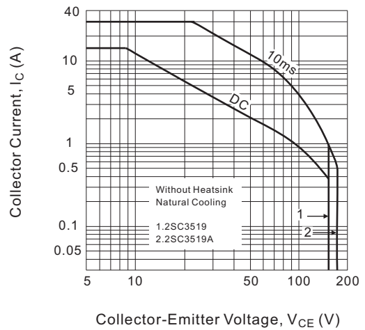
Fig.8 Safe Operating Area (Single Pulse)
