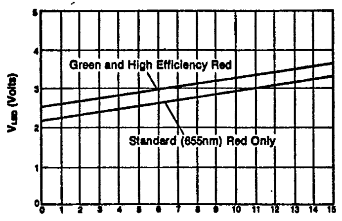
FIGURE 3—Min V_{LED} vs Drive Current Per LED
