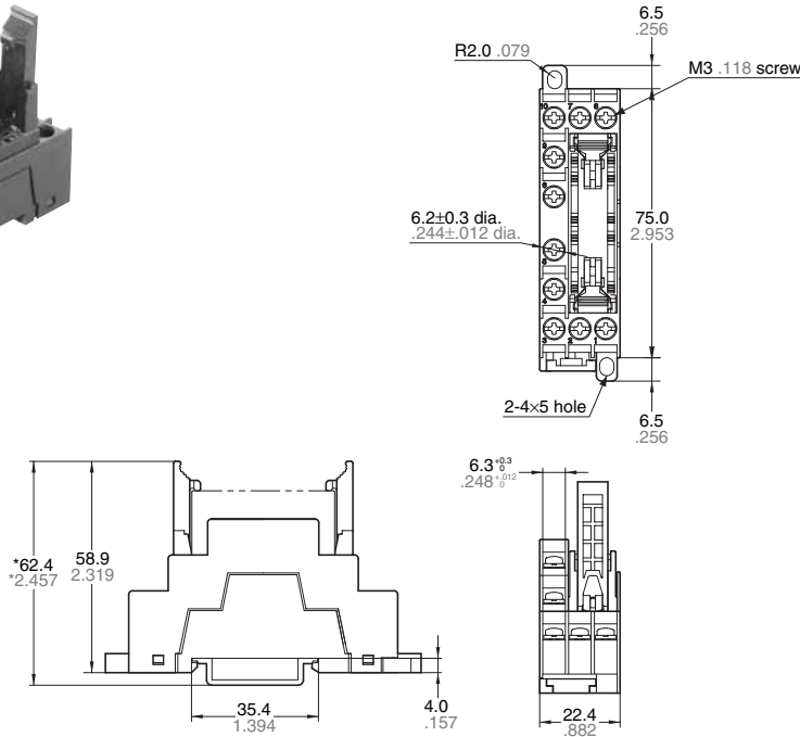
External dimensions
