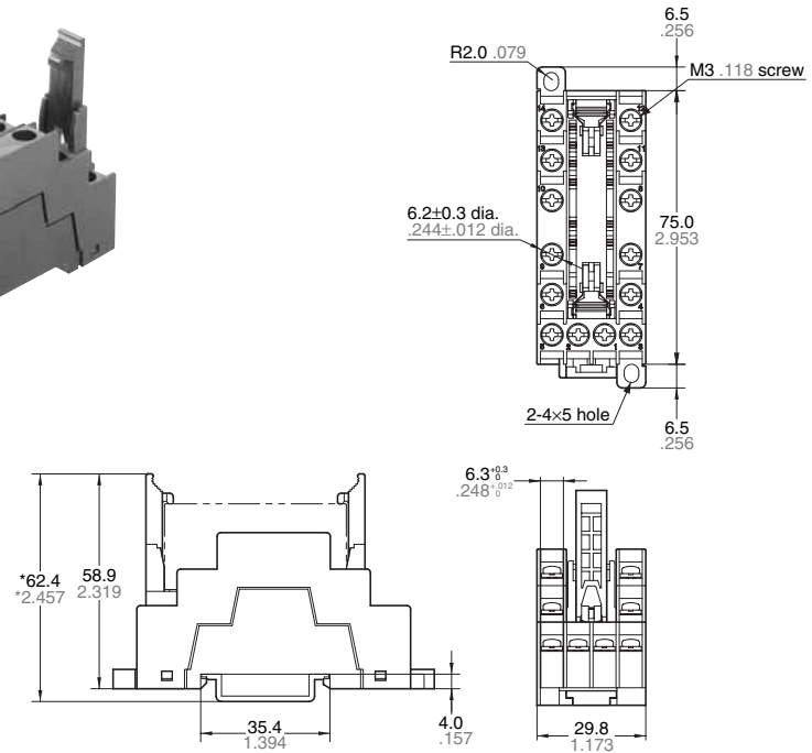
External dimensions
