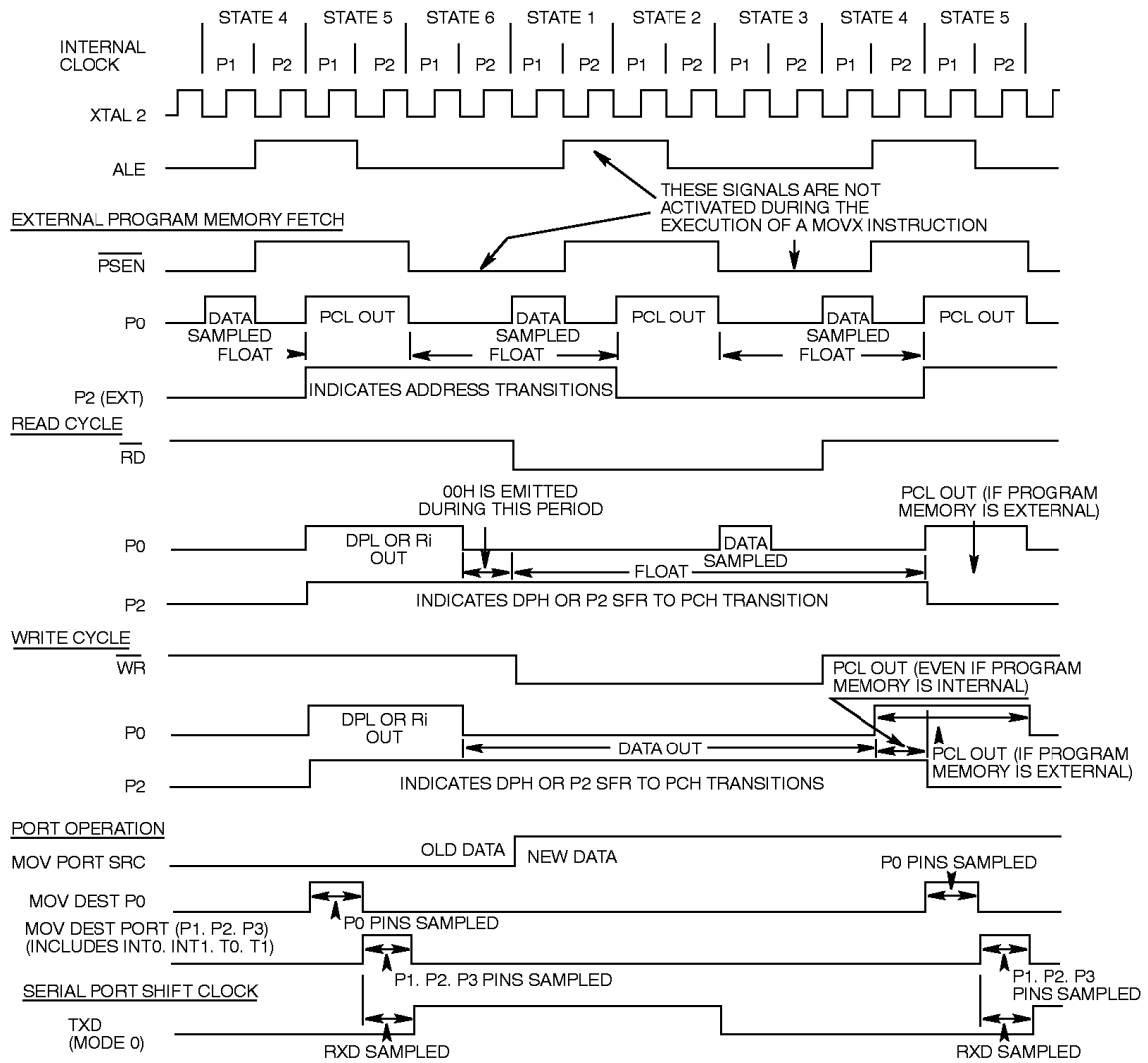
Figure 20. Clock Waveforms
