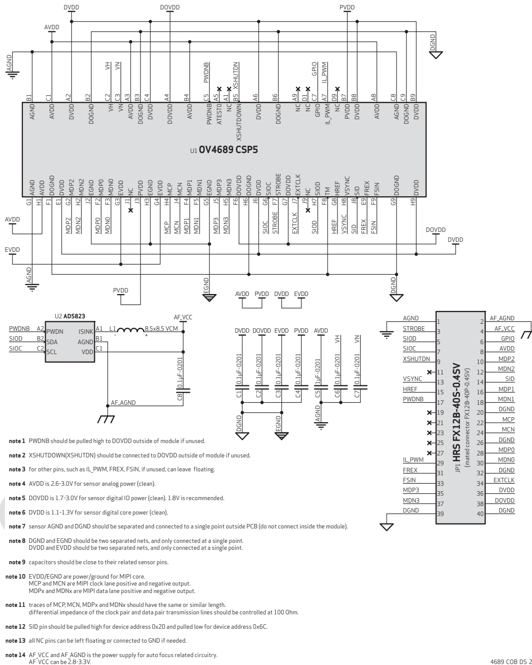
figure 2-2 reference schematic
