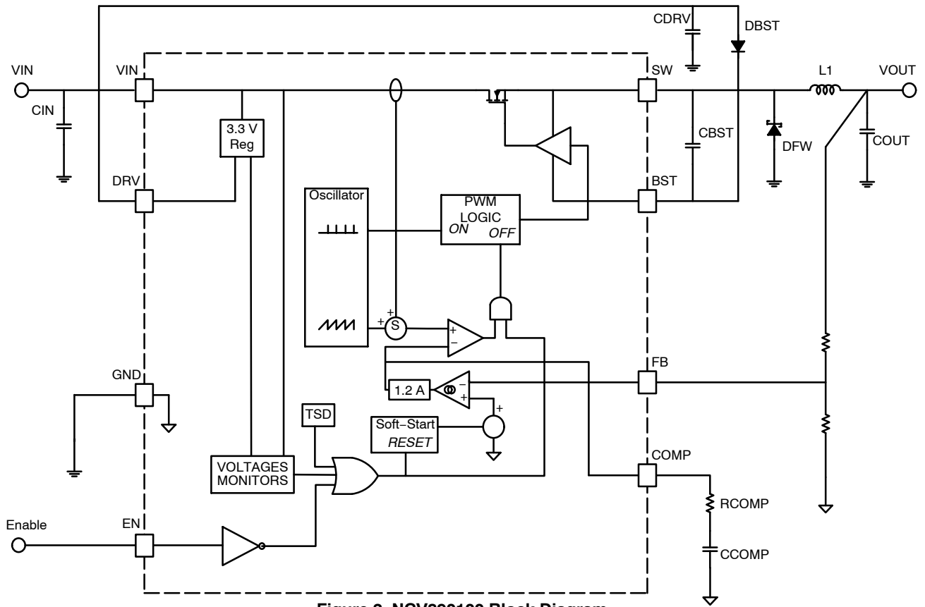
Figure 2. NCV890100 Block Diagram
