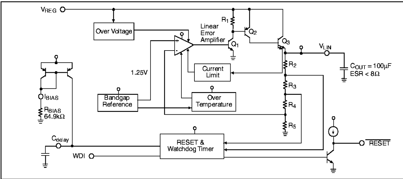
Figure 2. Block diagram of 5V linear regulator portion of the CS-5111.
