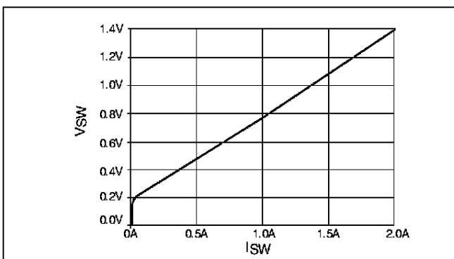
Figure 1c. Switch Saturation Voltage
