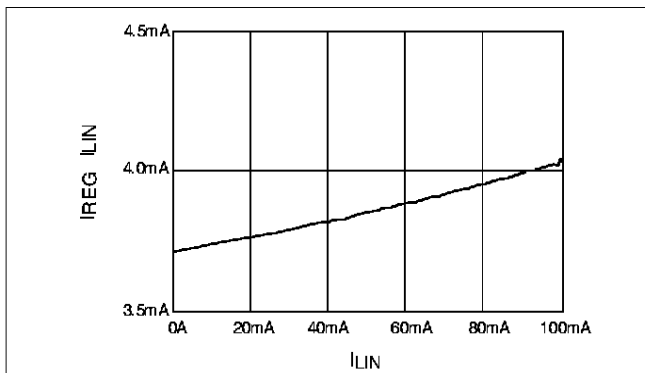
Figure 1a. 5V Regulator Bias Current vs. Load Current
