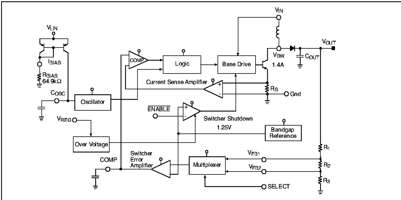
Figure 6: Block diagram of the 1.4A current mode control switching regulator portion of the CS-5111 in a boost configuration.
