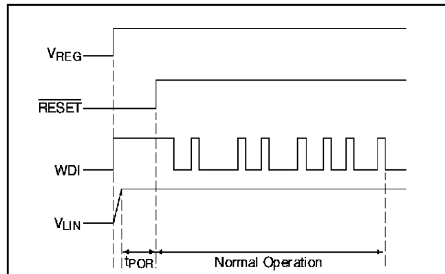
Figure 3. Timing diagram for normal regulator operation.
