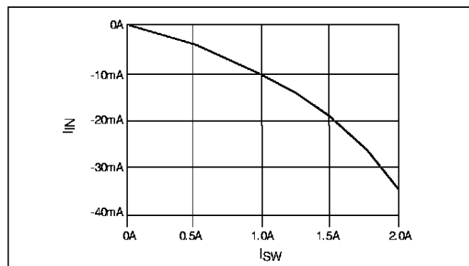
Figure 1b. Supply Current vs. Switch Current
