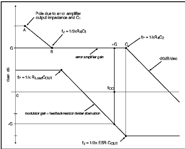
Figure 10. Bode plot of error amplifier (OTA) gain and modulator gain added to the feedback resistor divider attenuation.
