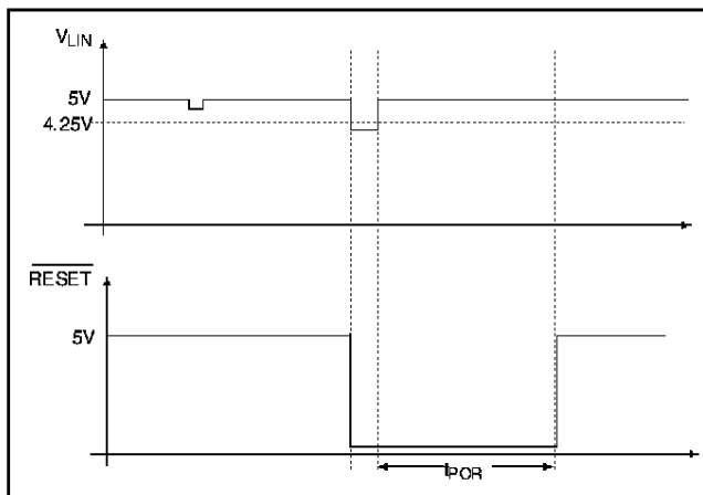
Figure 5b. \overline{\text{RESET}} signal is issued whenever V_{\text{LIN}} falls below 4.25V (typical).
