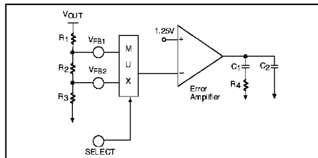
Figure 9. RC network used to compensate the error amplifier (OTA).
