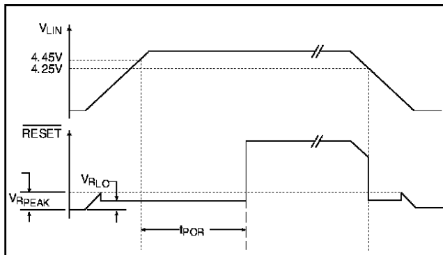
Figure 5a. The power on reset time interval ( t_{\text{POR}} ) begins when V_{\text{LIN}} rises above 4.45V (typical).
