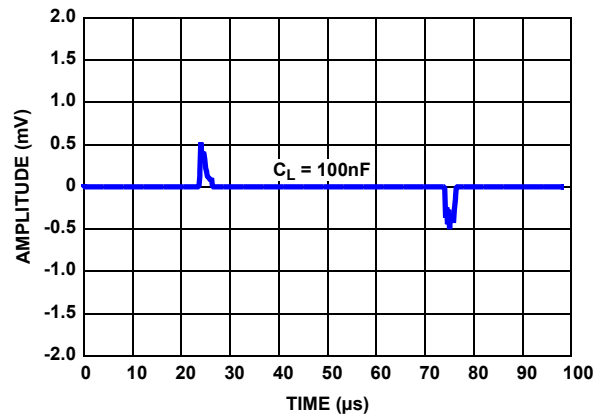
FIGURE 8. LINE TRANSIENT WITH 100nF LOAD ( \Delta V_{IN} = \pm 500mV )
