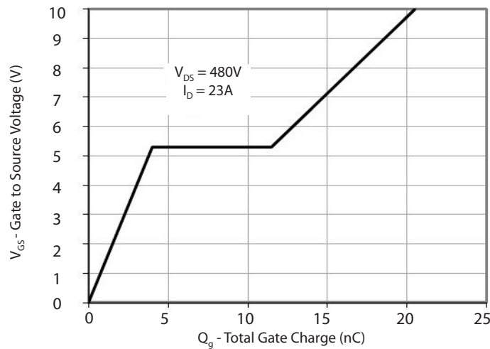
Gate Charge
