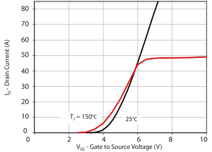
Transfer Characteristics
