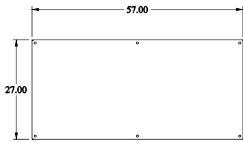
INNER PANEL
