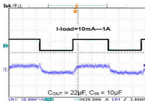
Load Transients
