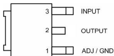
Package: TO-252
