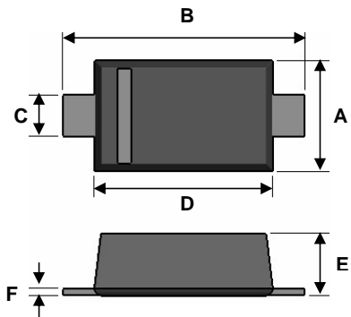
SOD-323
