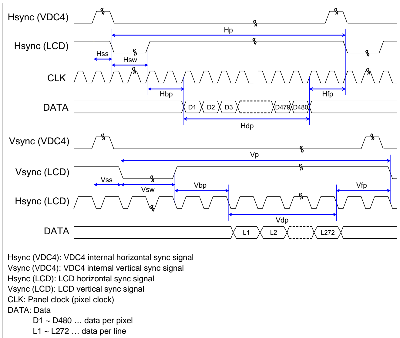
Figure 16 Signal Changing Timing of the LCD driven by Hsync and Vsync
