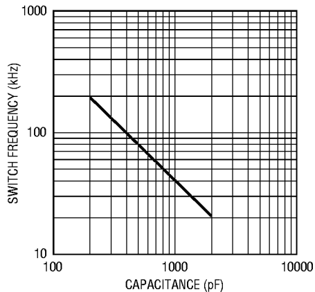
Switch Oscillator Frequency vs Capacitance
