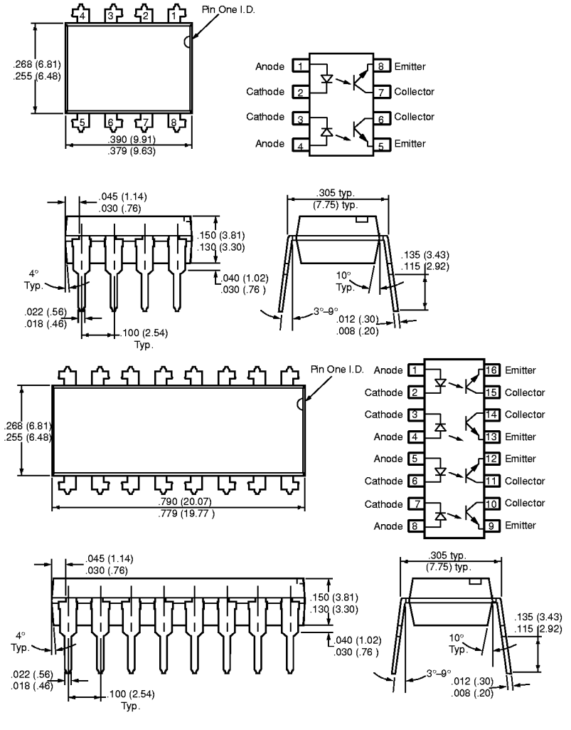
Dimensions in inches (mm)
