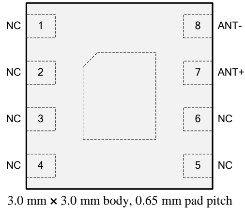
Top View (PCB Layout)
