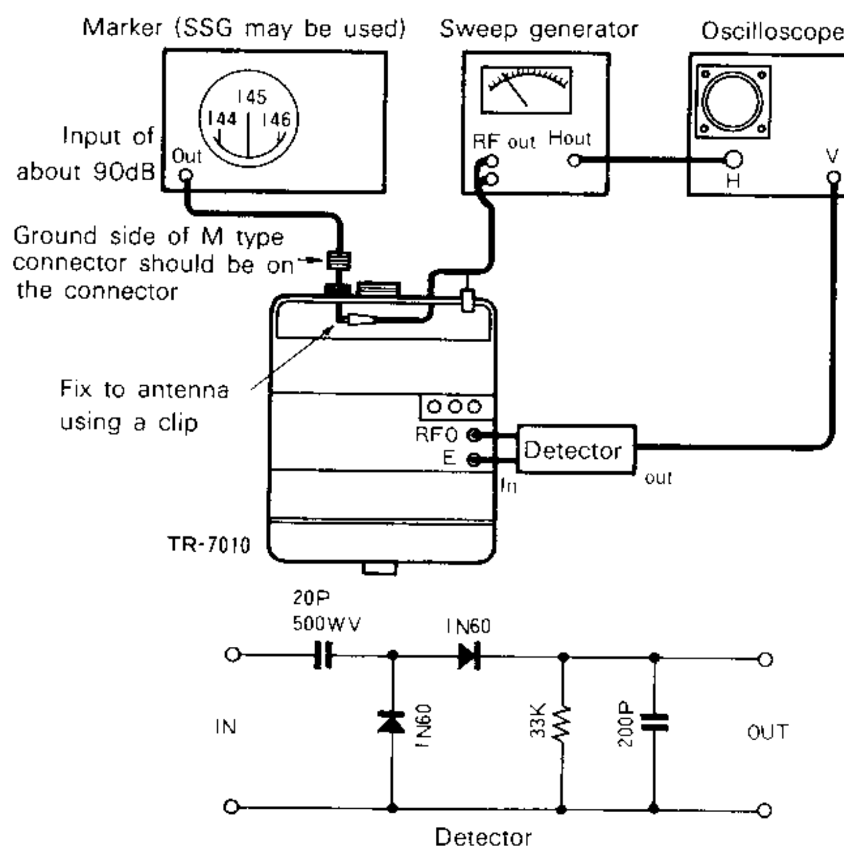
FIG. 12 HELICAL ADJUSTMENT
