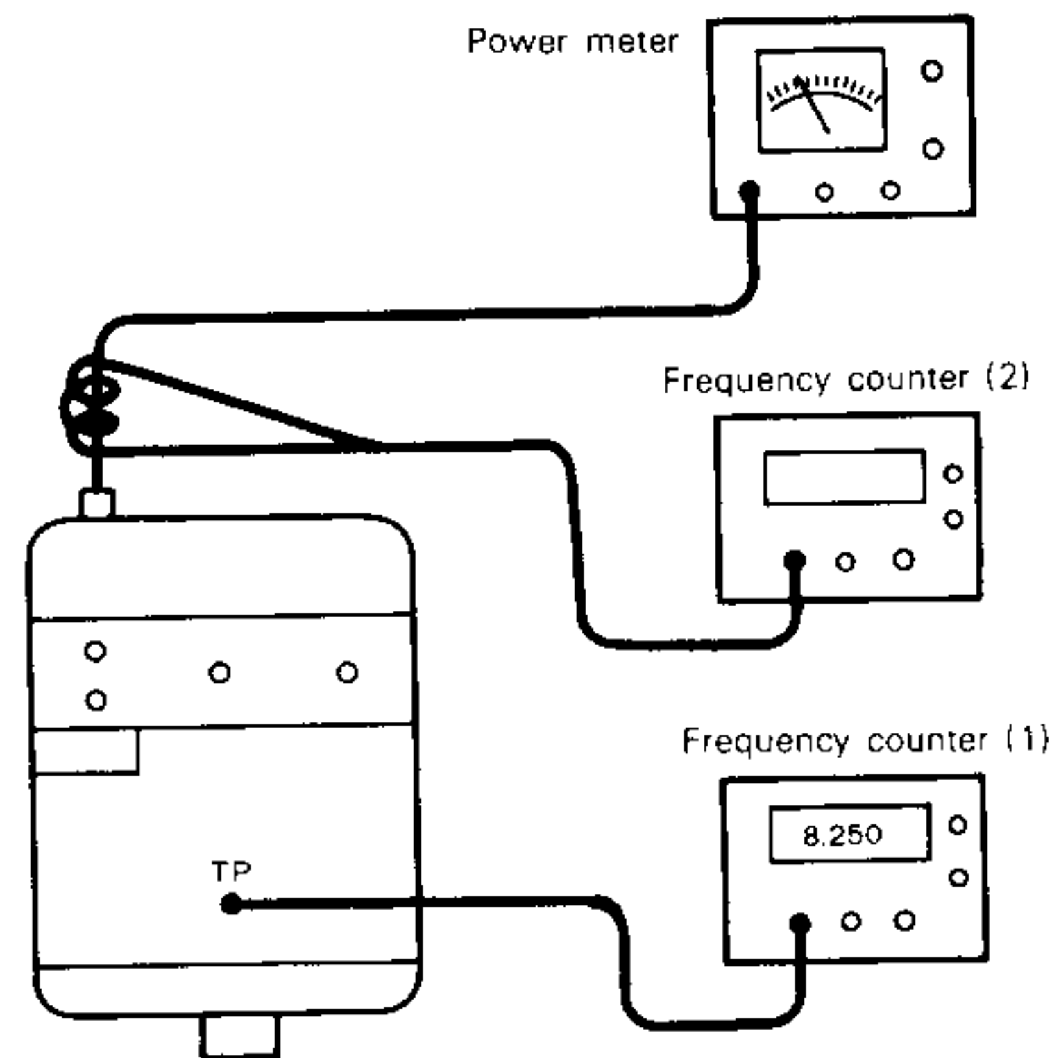
FIG. 19 FREQUENCY ADJUSTMENT
