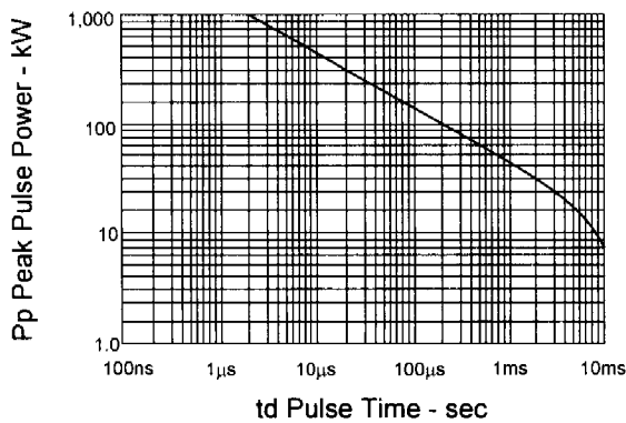
Fig. 3 - Peak Pulse Power vs. Pulse Time
