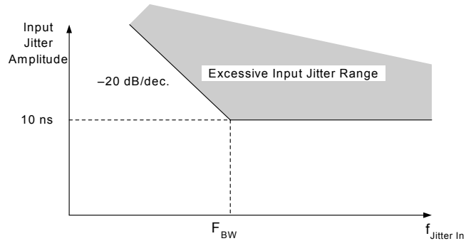
Figure 6. Jitter Tolerance Mask/Template
