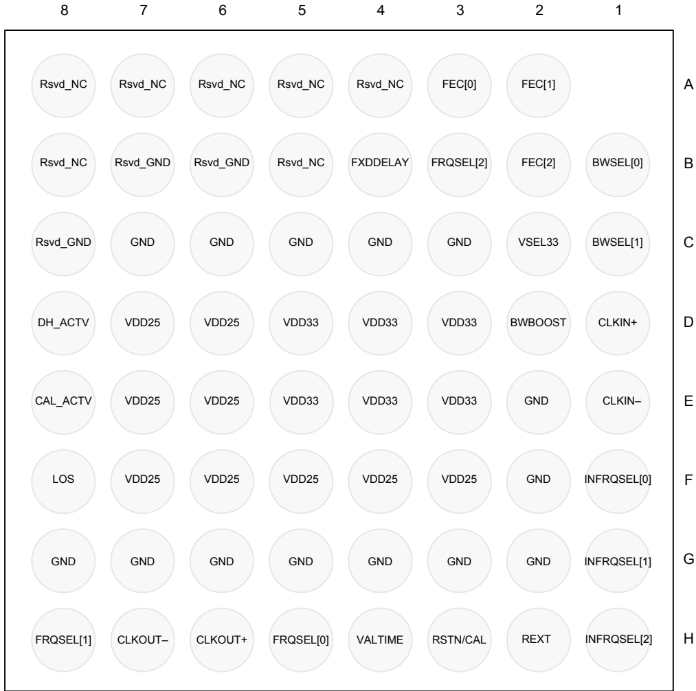
Bottom View
