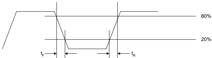
Figure 2. Rise/Fall Time Measurement
