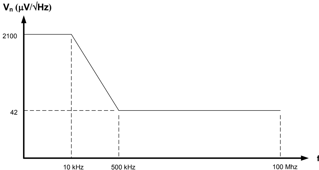
Figure 8. Power Supply Noise Tolerance Mask
