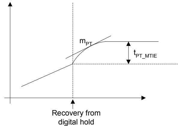
Figure 7. Recovery from Digital Hold
