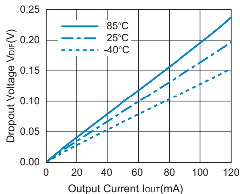
R1141Q281x Dropout Voltage vs. Output Current
