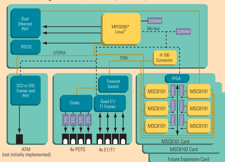
Reference Design Overview (with future expansion cards)
