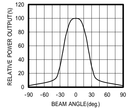
RADIATION PATTERN
